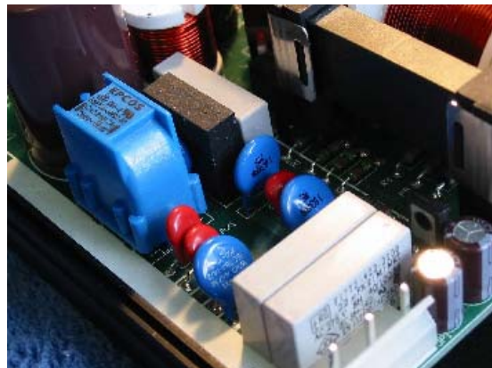
Close up of RFI & Transient protection circuit
